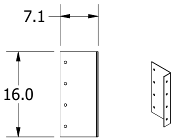
Optional WMB02 Wall Bracket Short
