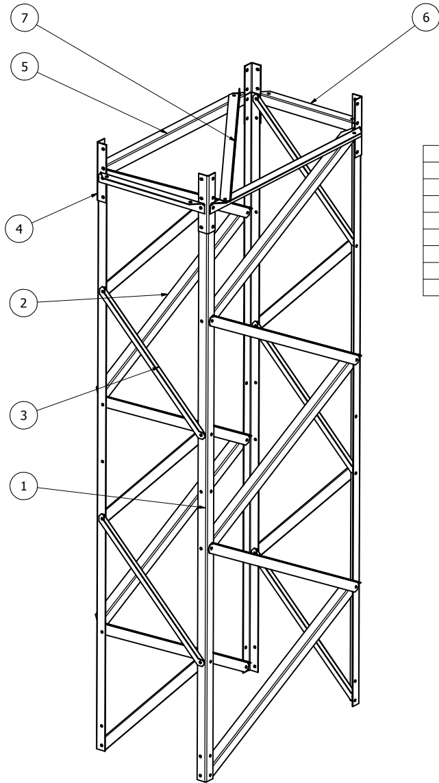
T48278 8 ga Tower odd sections
