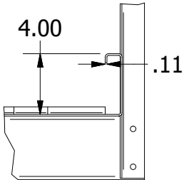
DETAIL A SCALE 1 / 9
